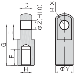
HCPM-IP040
