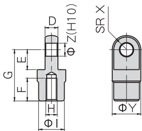
HCPM-IP020、HCPM-IP025
