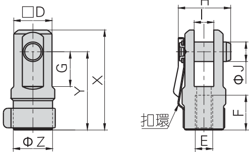
HCPM-YT020P、HCPM-YT025P
