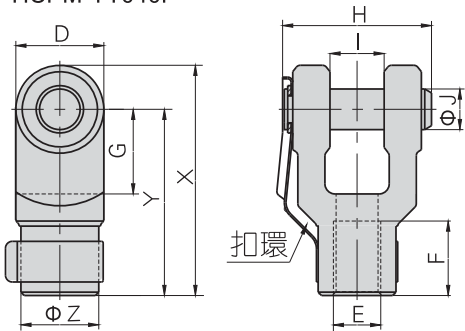
HCPM-YT040P
